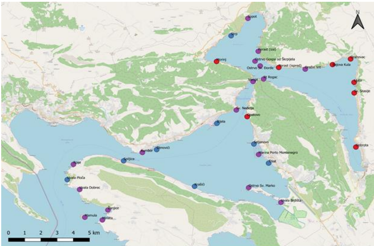
Figure 1. Sampling Locations: Red-personal data, Purple-personal and literature data, Blue-literature data
